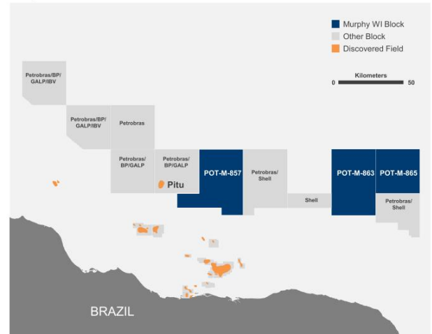
Potiguar Basin
