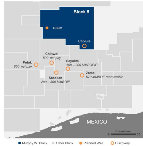
Salina Basin
