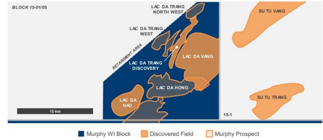
Cuu Long Basin
