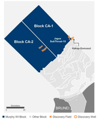
Northwest Borneo Basin
