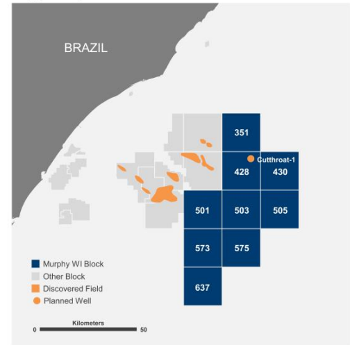
Sergipe-Alagoas Basin
